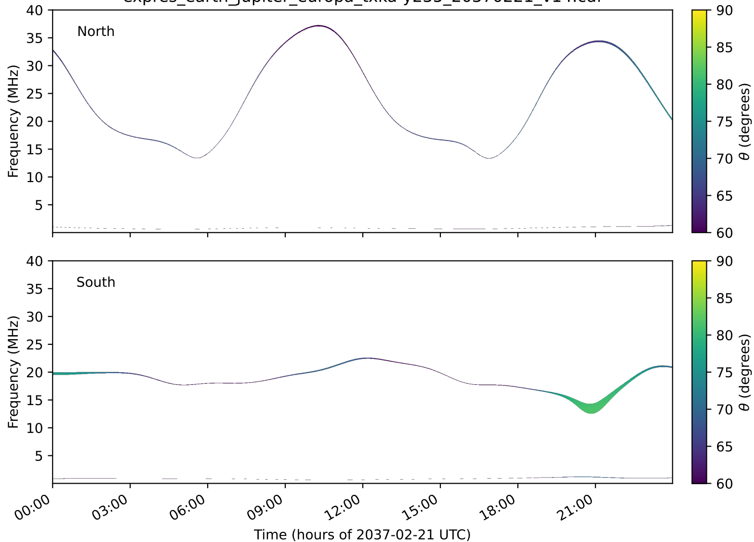
expres_earth_jupiter_europa_txka-y235_20370221_v14.cdf
