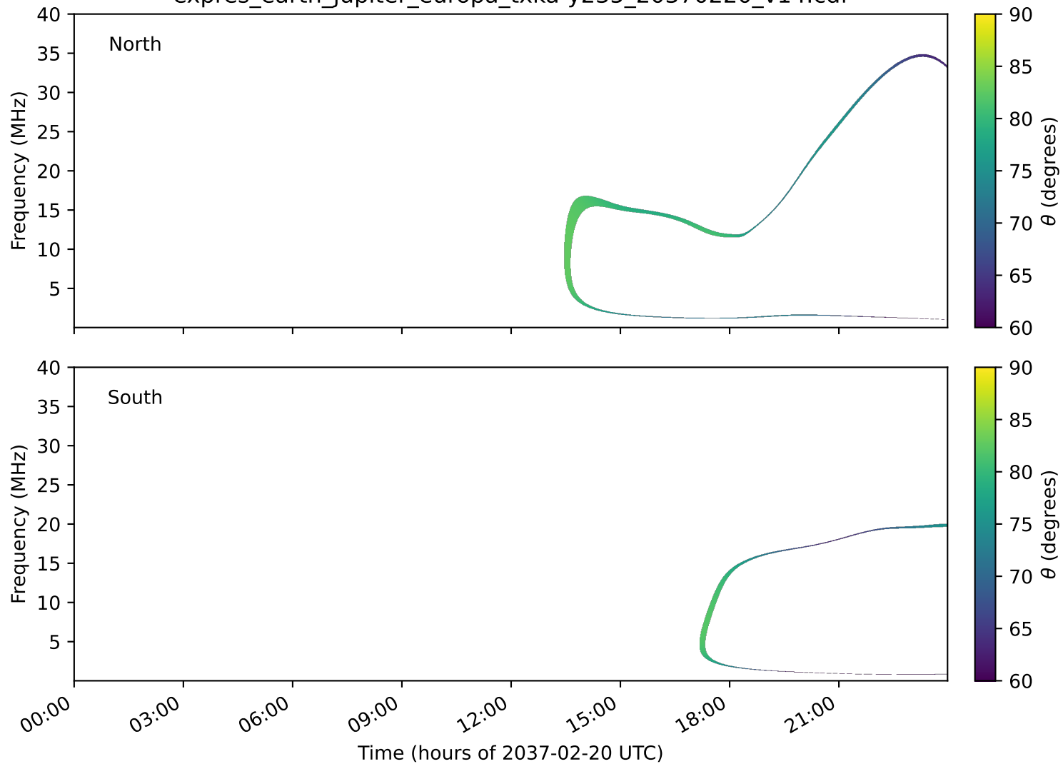
expres_earth_jupiter_europa_txka-y235_20370220_v14.cdf
