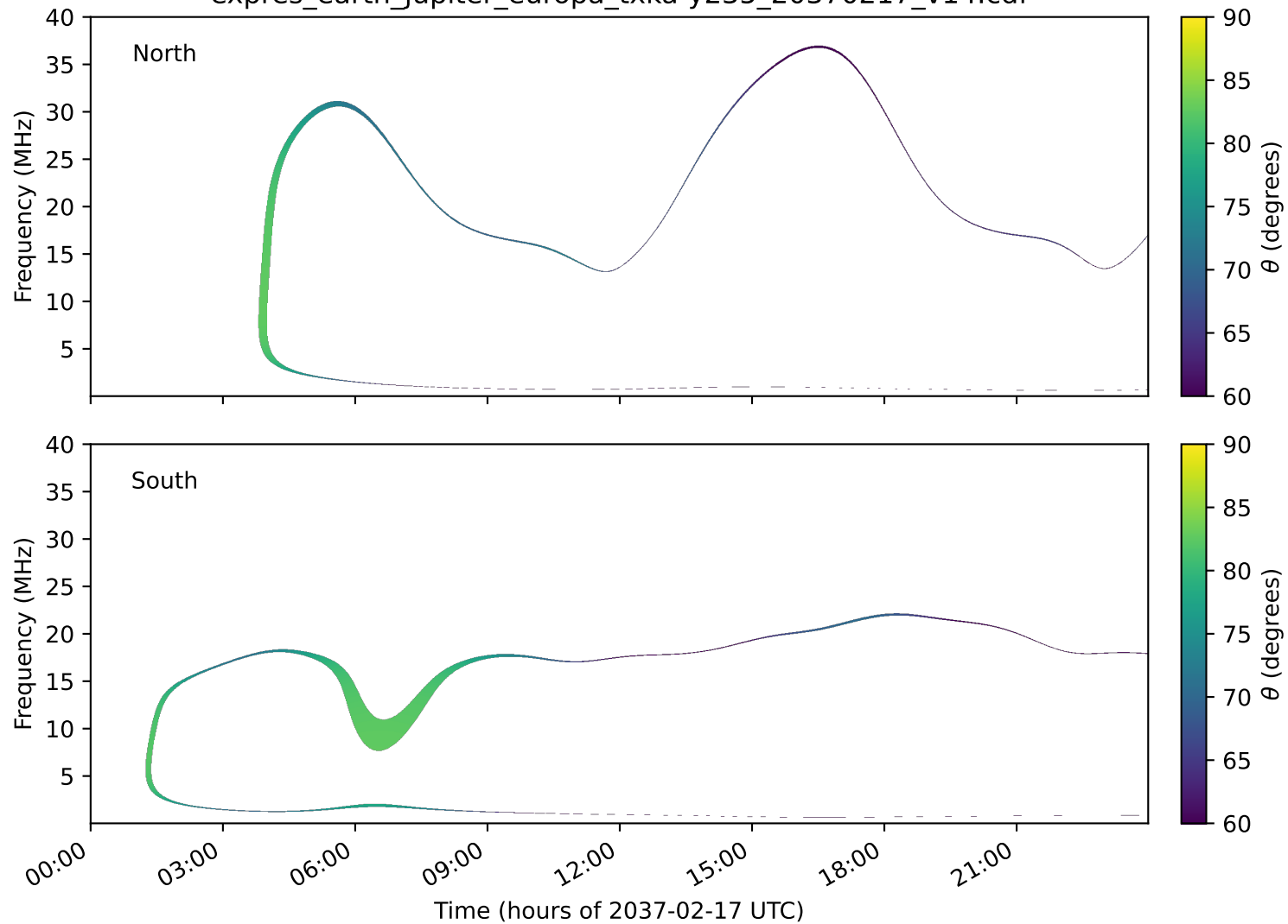
expres_earth_jupiter_europa_txka-y235_20370217_v14.cdf
