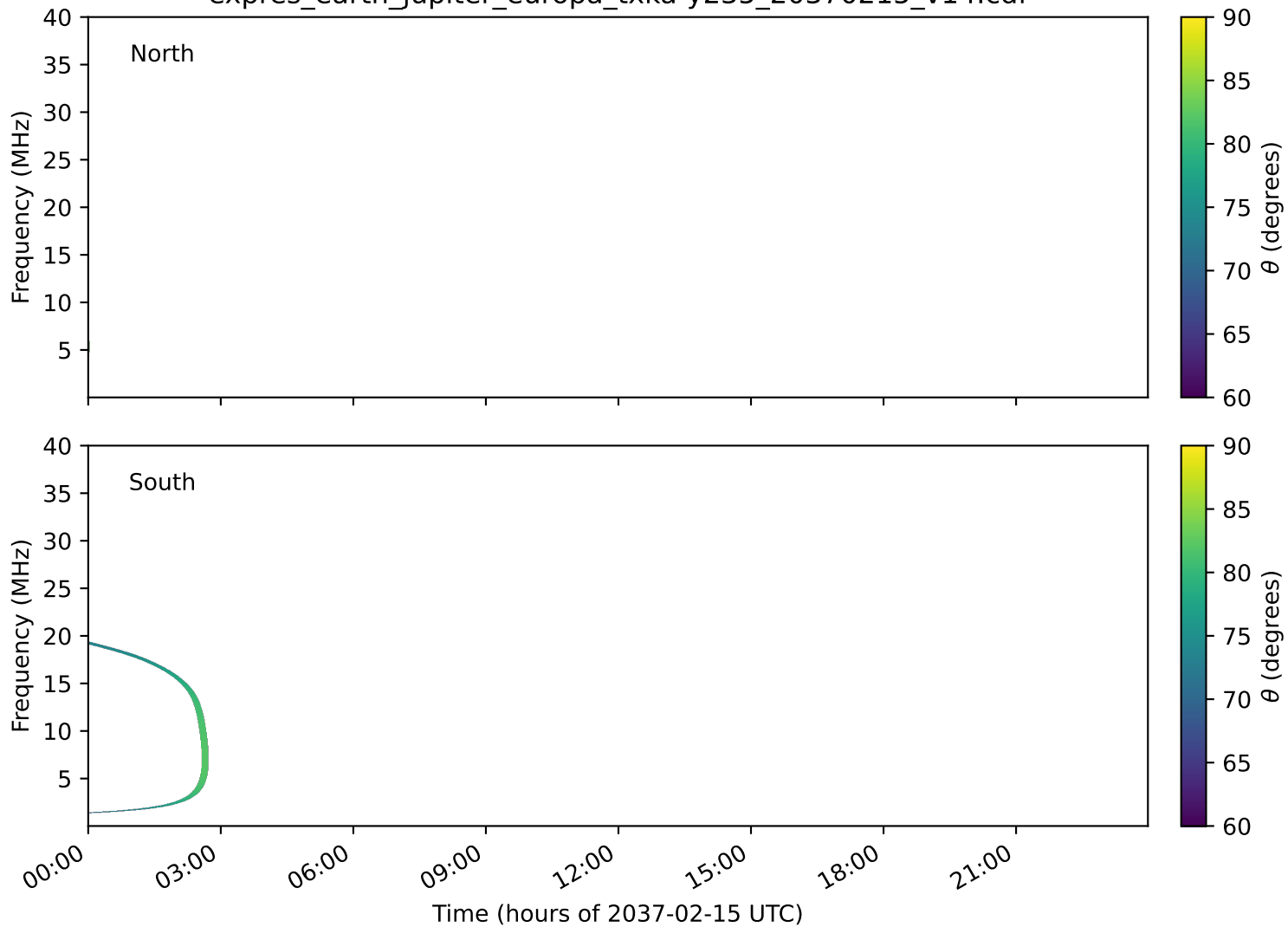
expres_earth_jupiter_europa_txka-y235_20370215_v14.cdf
