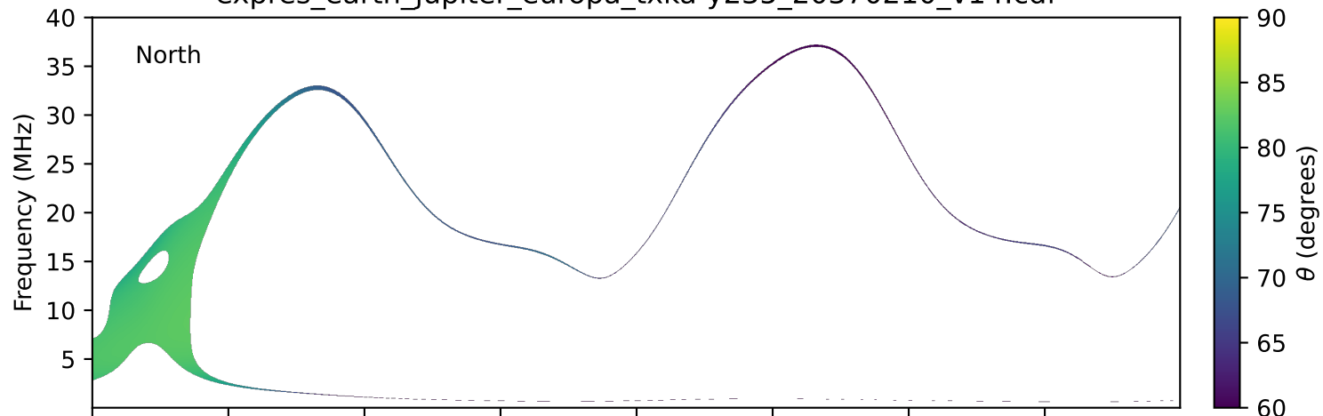
expres_earth_jupiter_europa_txka-y235_20370210_v14.cdf
