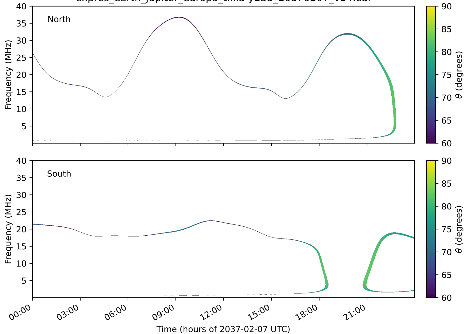
expres_earth_jupiter_europa_txka-y235_20370207_v14.cdf
