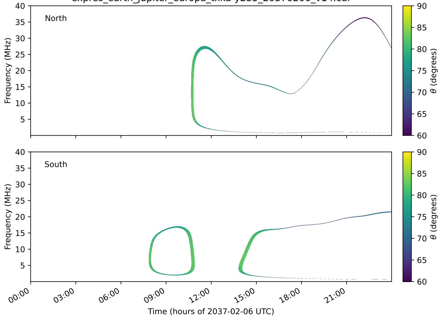
expres_earth_jupiter_europa_txka-y235_20370206_v14.cdf
