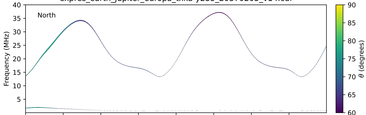
expres_earth_jupiter_europa_txka-y235_20370203_v14.cdf
