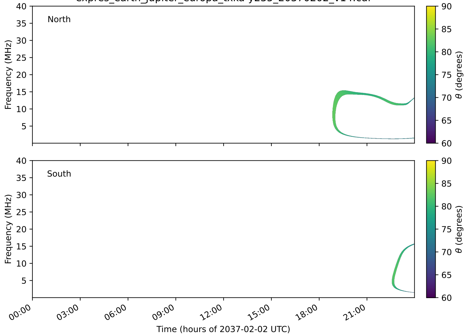
expres_earth_jupiter_europa_txka-y235_20370202_v14.cdf
