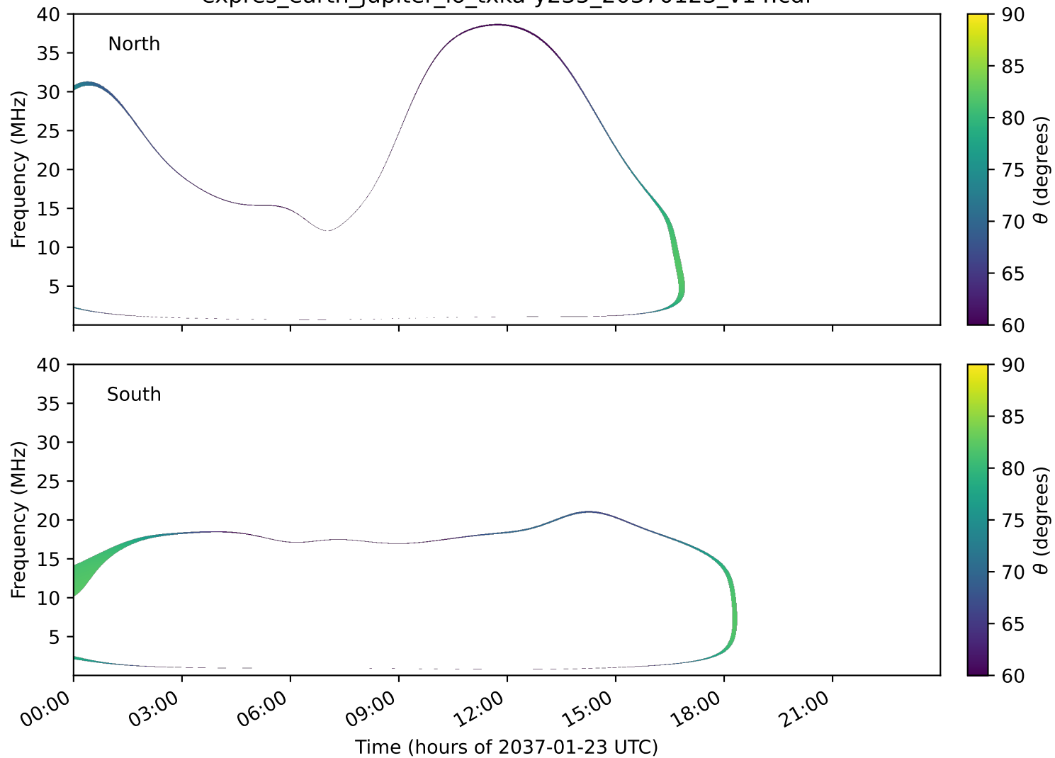
expres_earth_jupiter_io_txka-y235_20370123_v14.cdf
