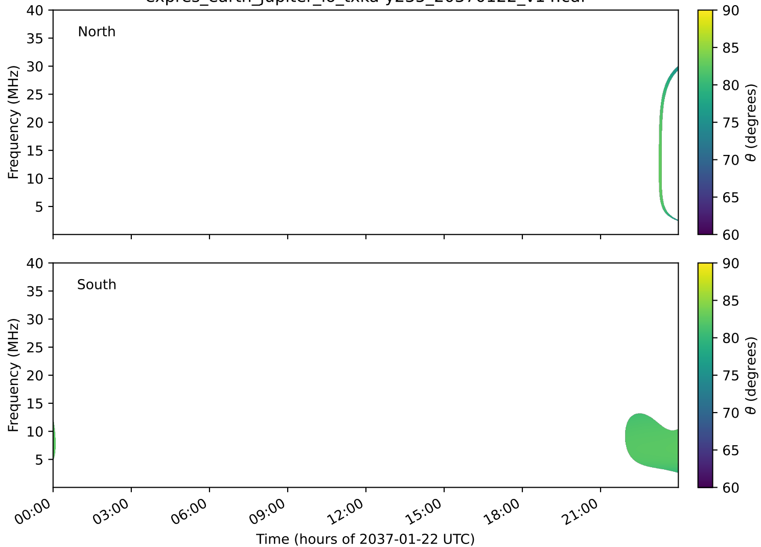
expres_earth_jupiter_io_txka-y235_20370122_v14.cdf
