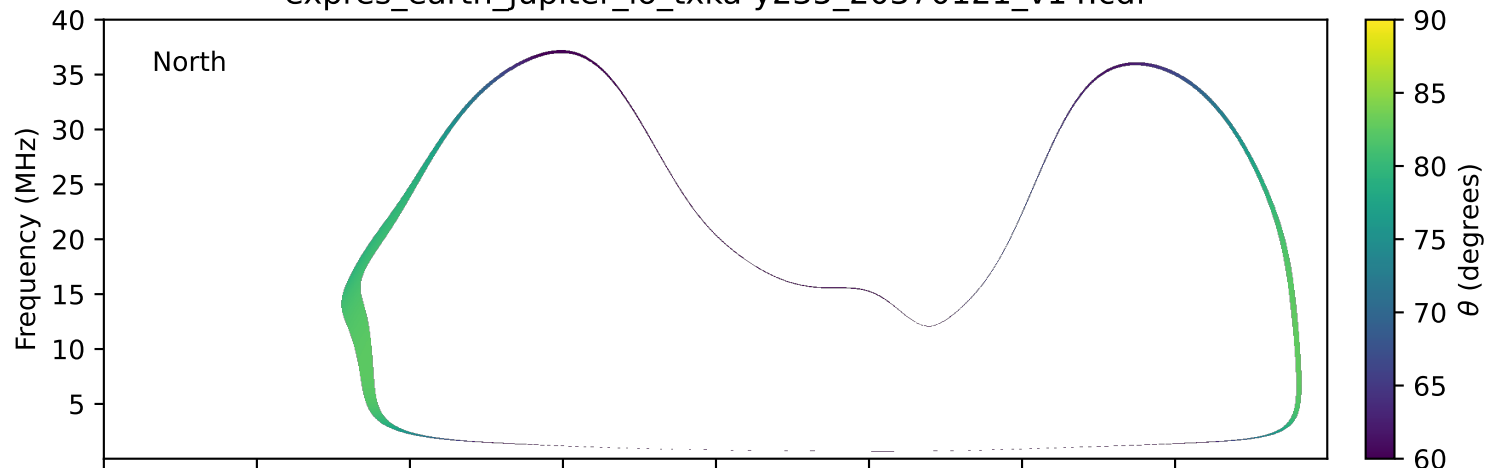
expres_earth_jupiter_io_txka-y235_20370121_v14.cdf
