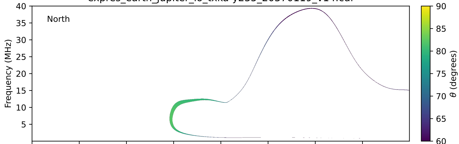
expres_earth_jupiter_io_txka-y235_20370119_v14.cdf
