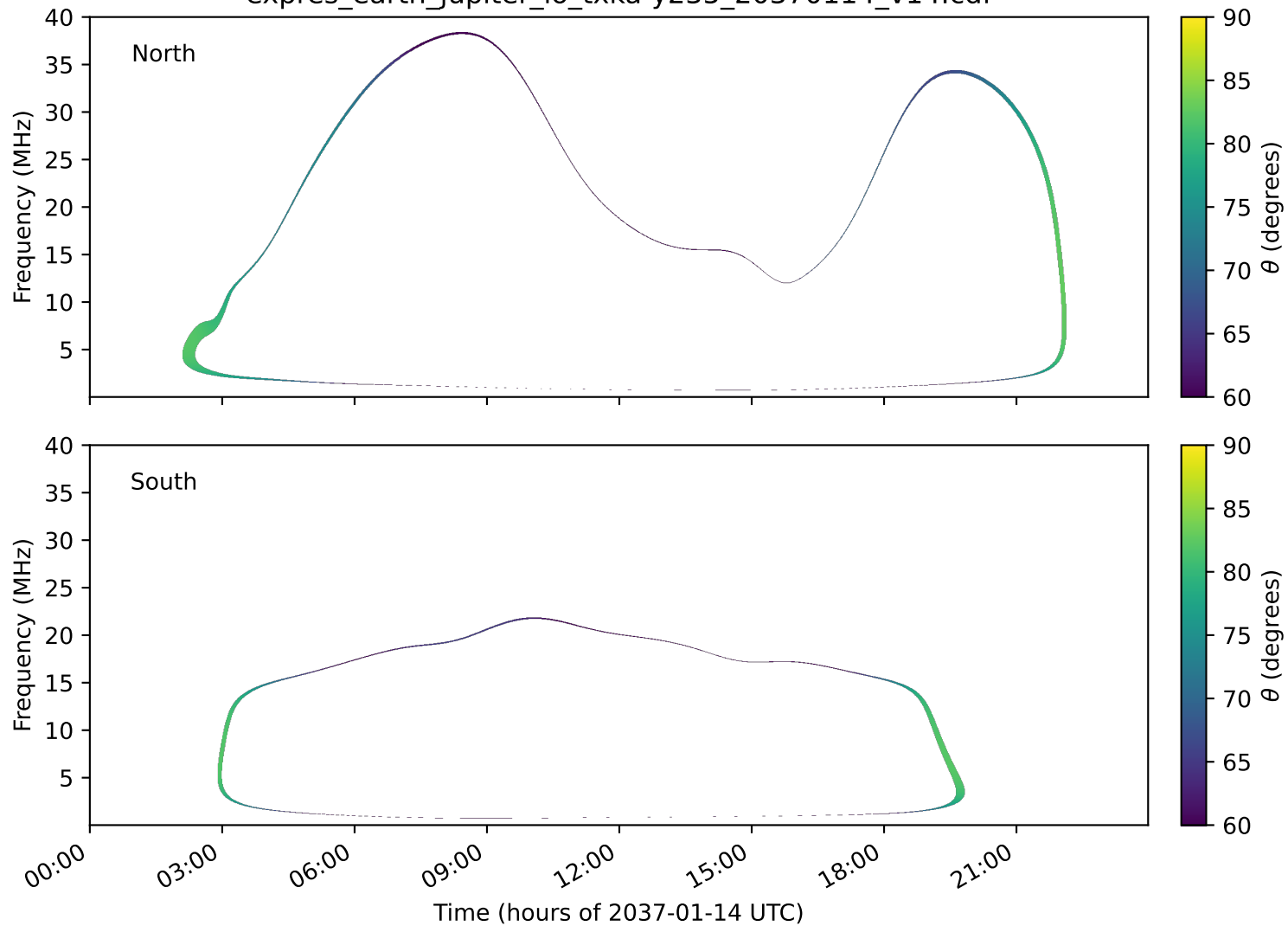
expres_earth_jupiter_io_txka-y235_20370114_v14.cdf
