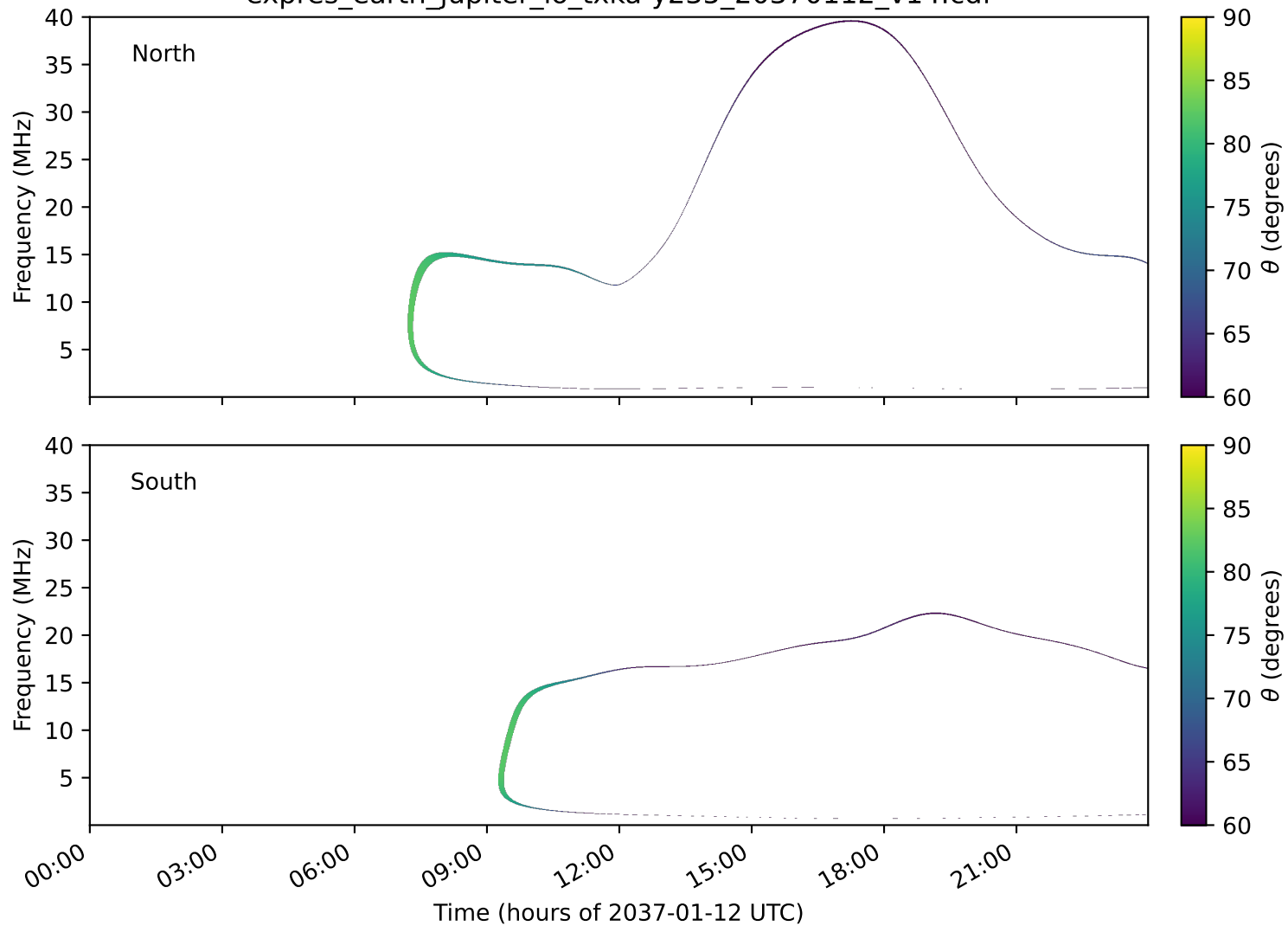
expres_earth_jupiter_io_txka-y235_20370112_v14.cdf
