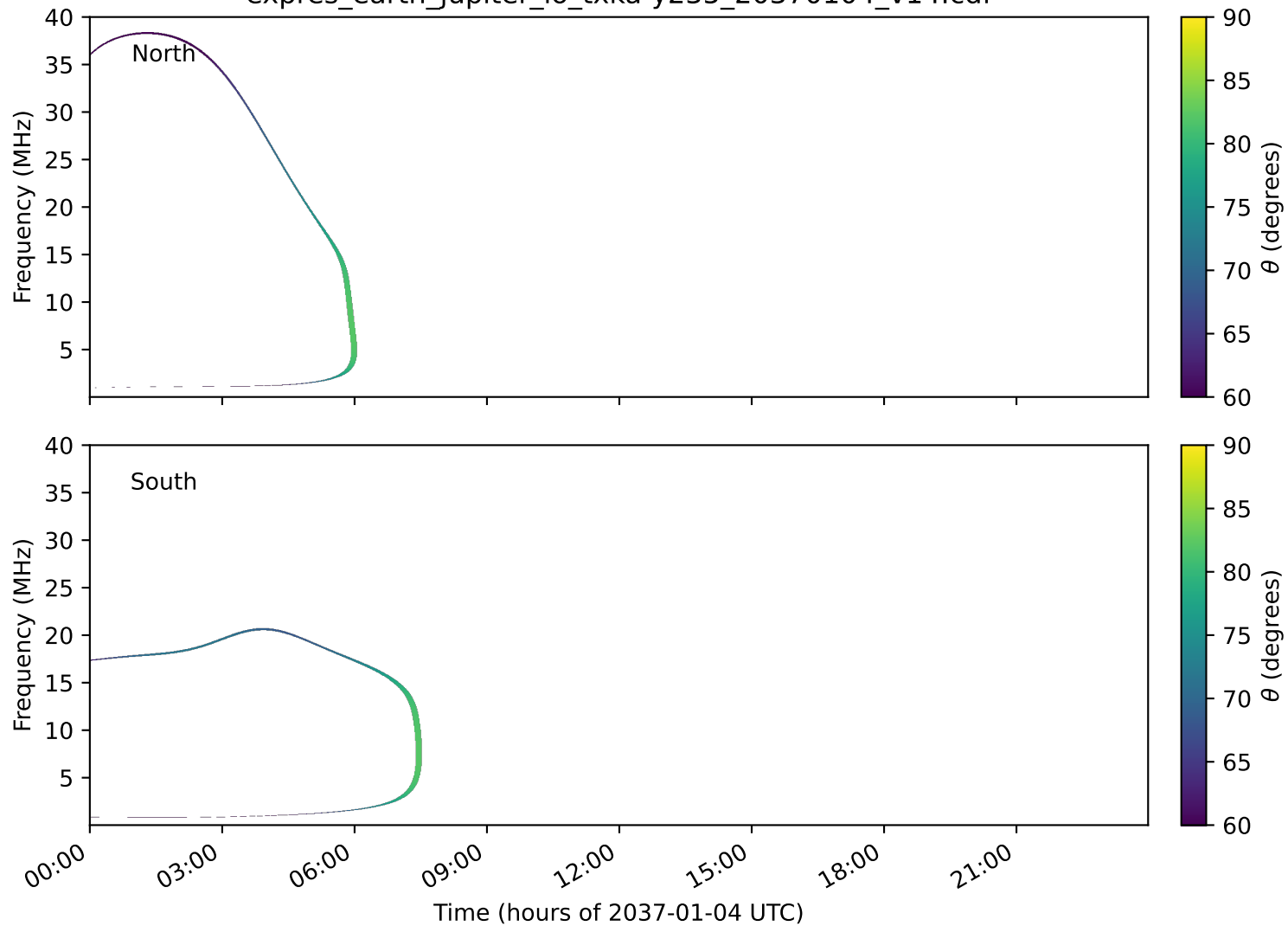
expres_earth_jupiter_io_txka-y235_20370104_v14.cdf
