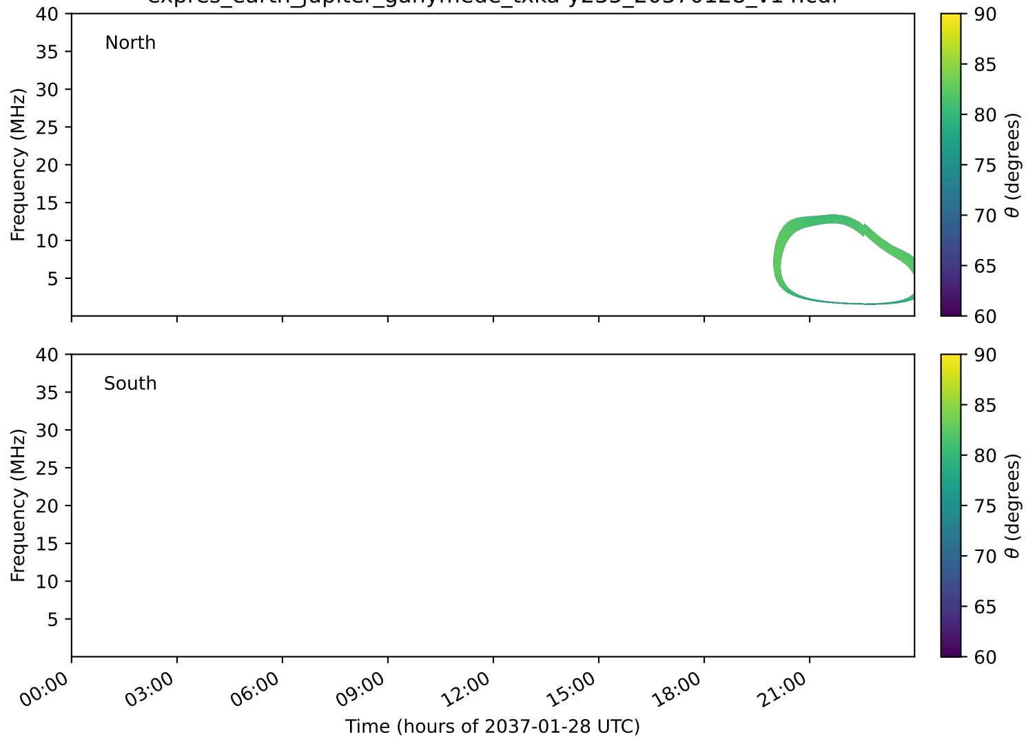
expres_earth_jupiter_ganymede_txka-y235_20370128_v14.cdf
