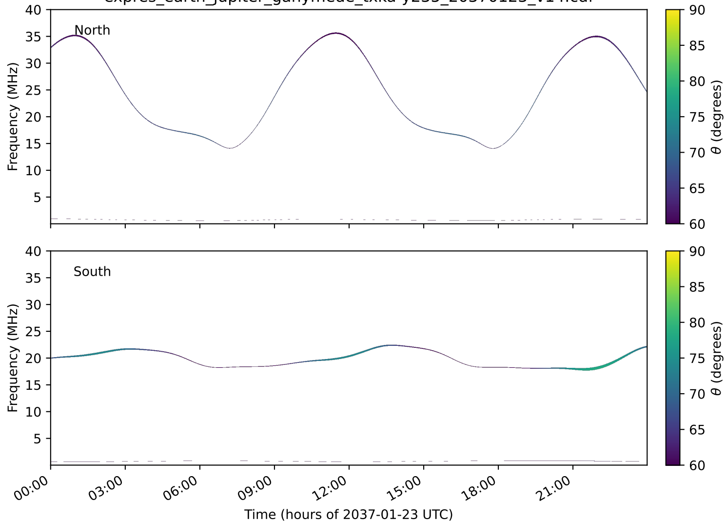
expres_earth_jupiter_ganymede_txka-y235_20370123_v14.cdf
