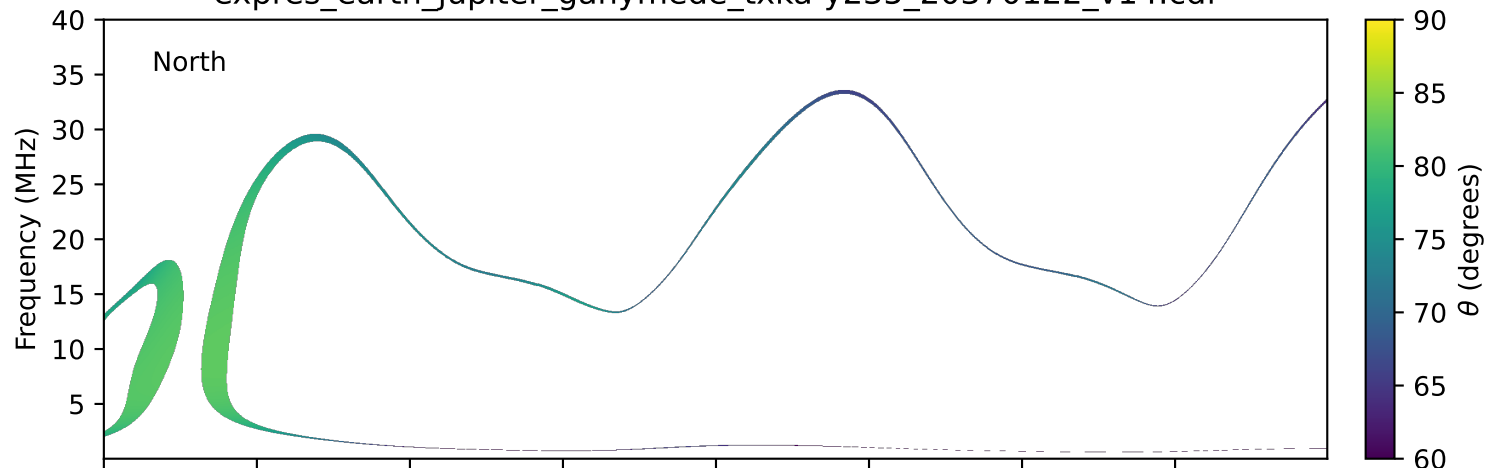
expres_earth_jupiter_ganymede_txka-y235_20370122_v14.cdf
