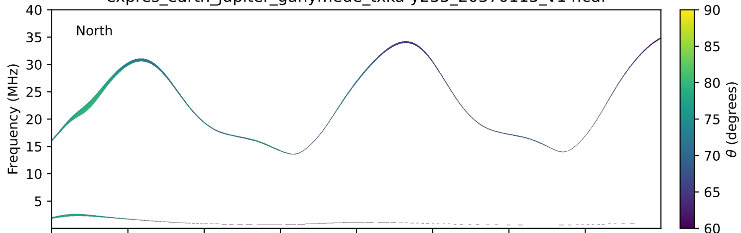
expres_earth_jupiter_ganymede_txka-y235_20370115_v14.cdf
