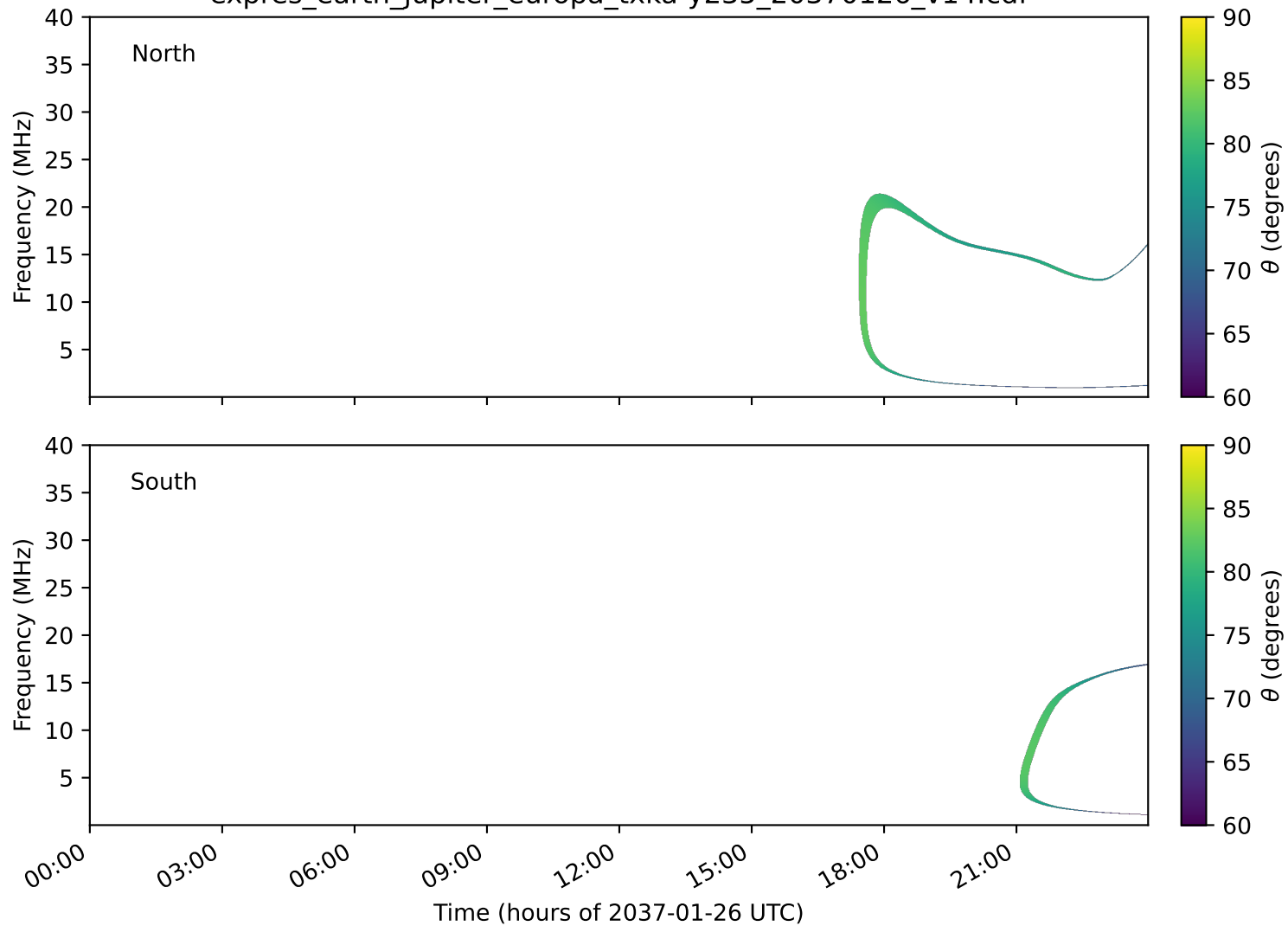
expres_earth_jupiter_europa_txka-y235_20370126_v14.cdf
