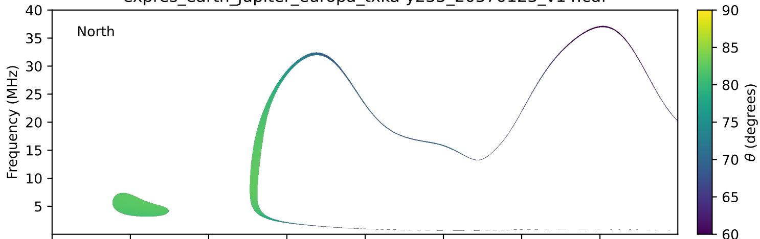
expres_earth_jupiter_europa_txka-y235_20370123_v14.cdf
