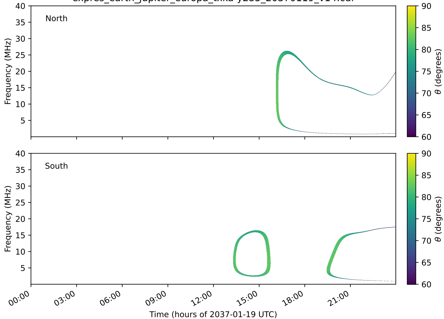
expres_earth_jupiter_europa_txka-y235_20370119_v14.cdf
