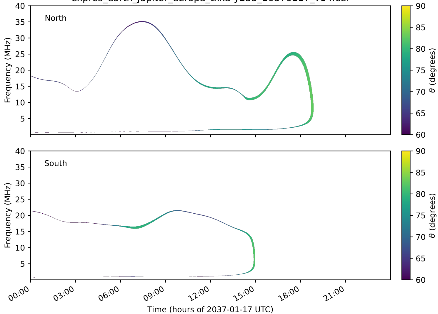
expres_earth_jupiter_europa_txka-y235_20370117_v14.cdf
