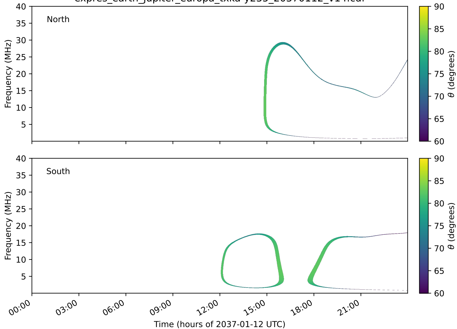
expres_earth_jupiter_europa_txka-y235_20370112_v14.cdf
