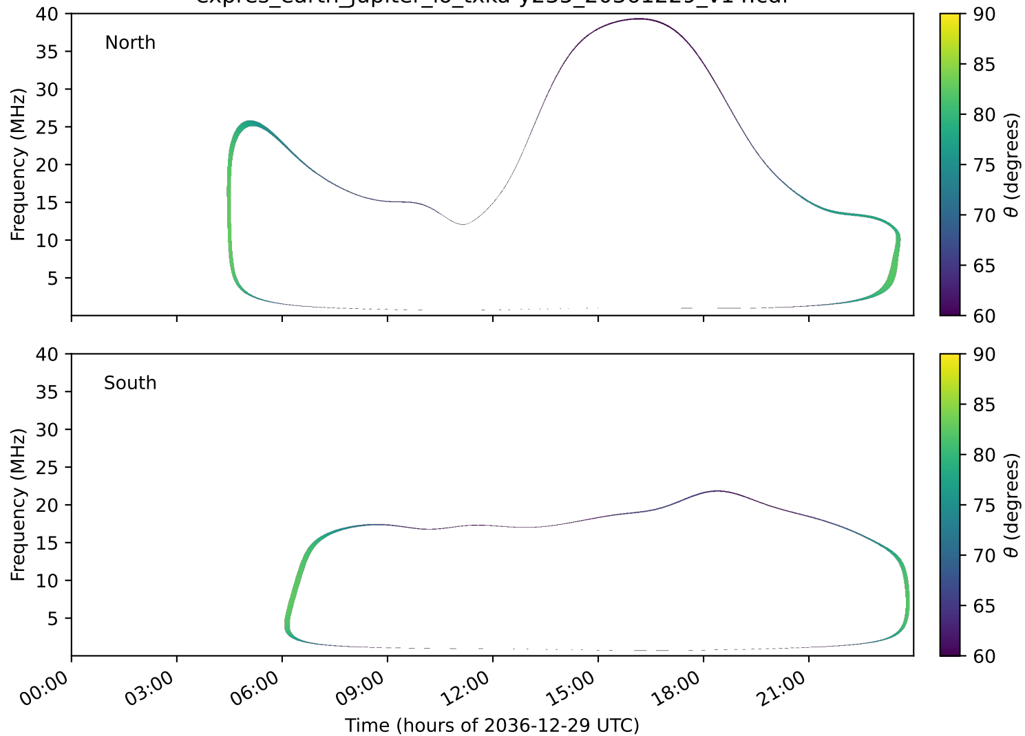
expres_earth_jupiter_io_txka-y235_20361229_v14.cdf
