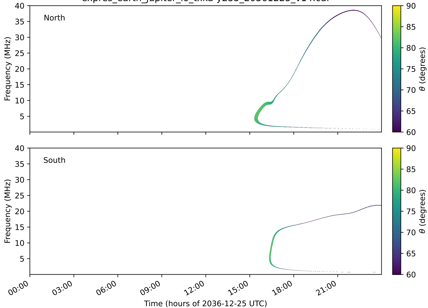
expres_earth_jupiter_io_txka-y235_20361225_v14.cdf
