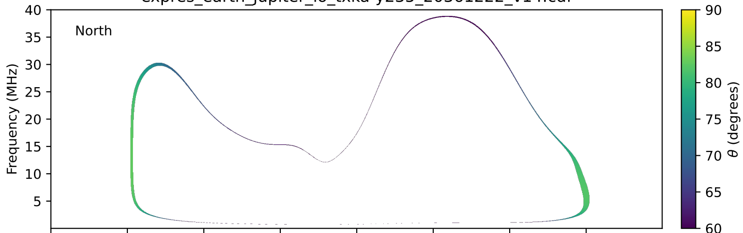
expres_earth_jupiter_io_txka-y235_20361222_v14.cdf
