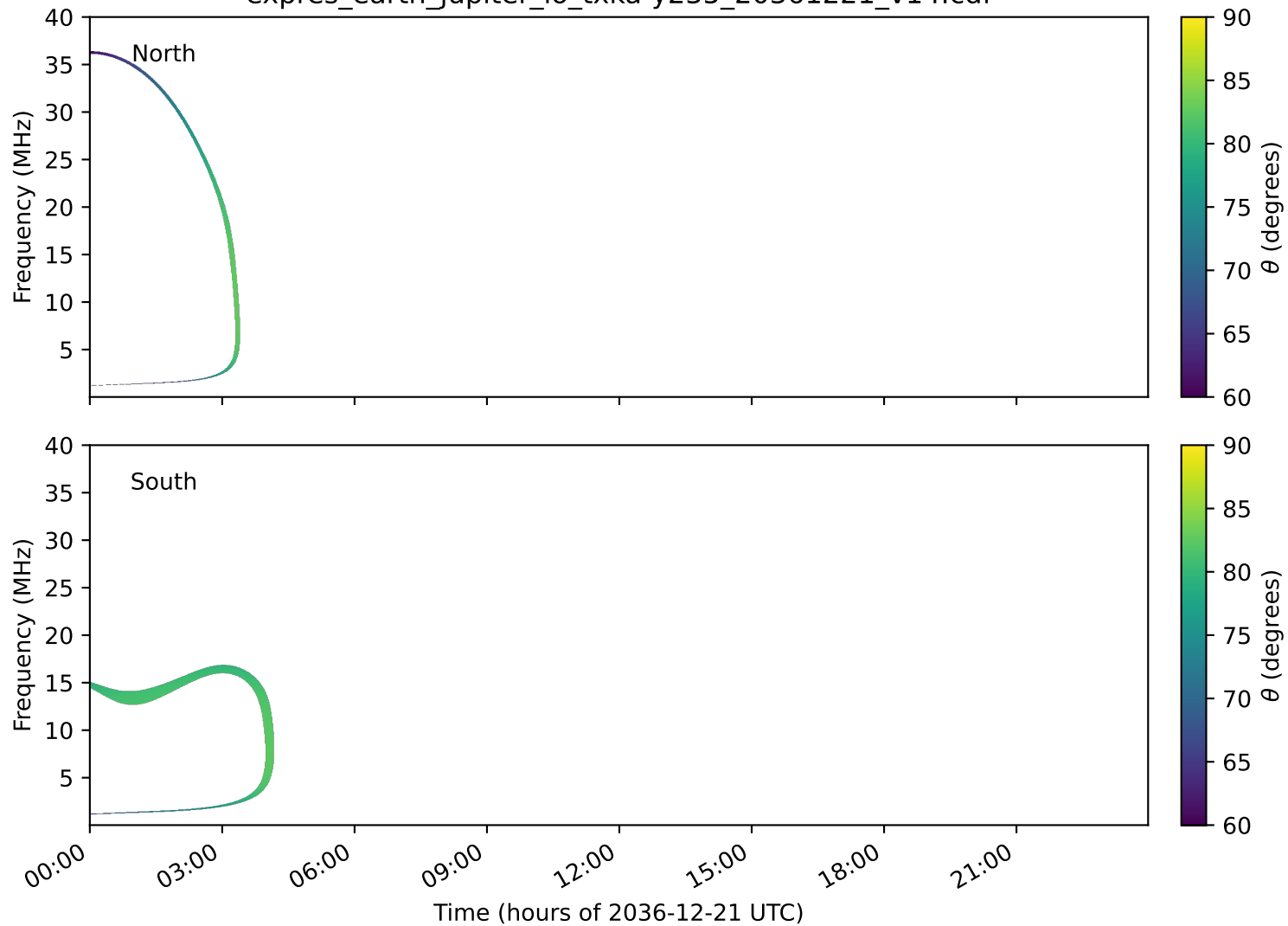
expres_earth_jupiter_io_txka-y235_20361221_v14.cdf
