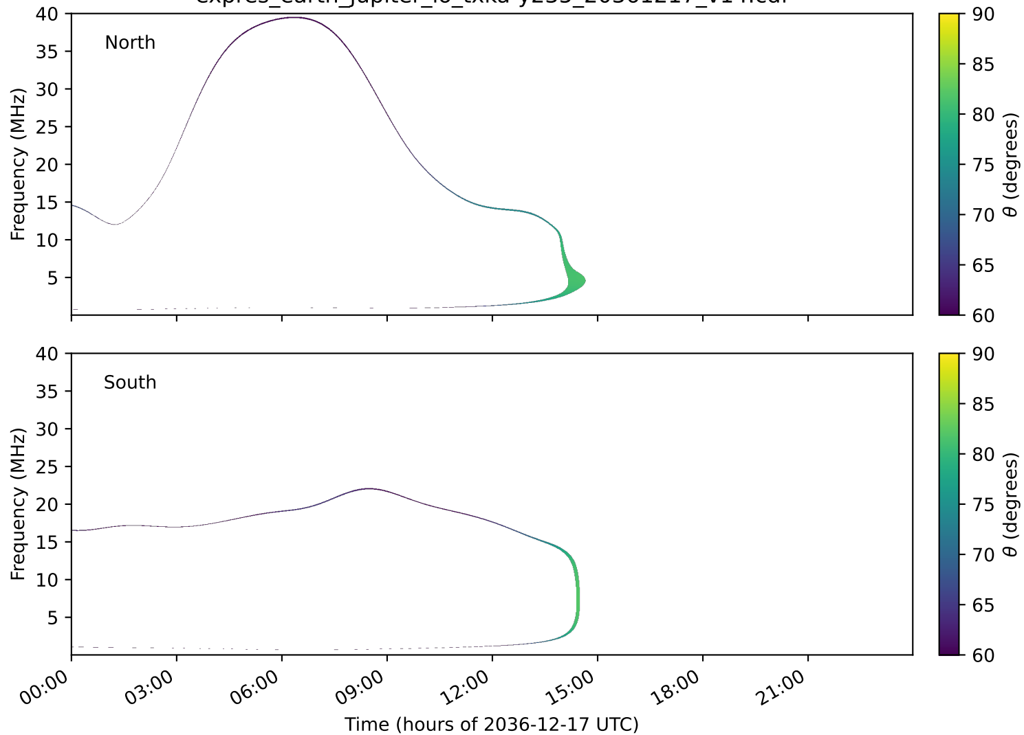
expres_earth_jupiter_io_txka-y235_20361217_v14.cdf
