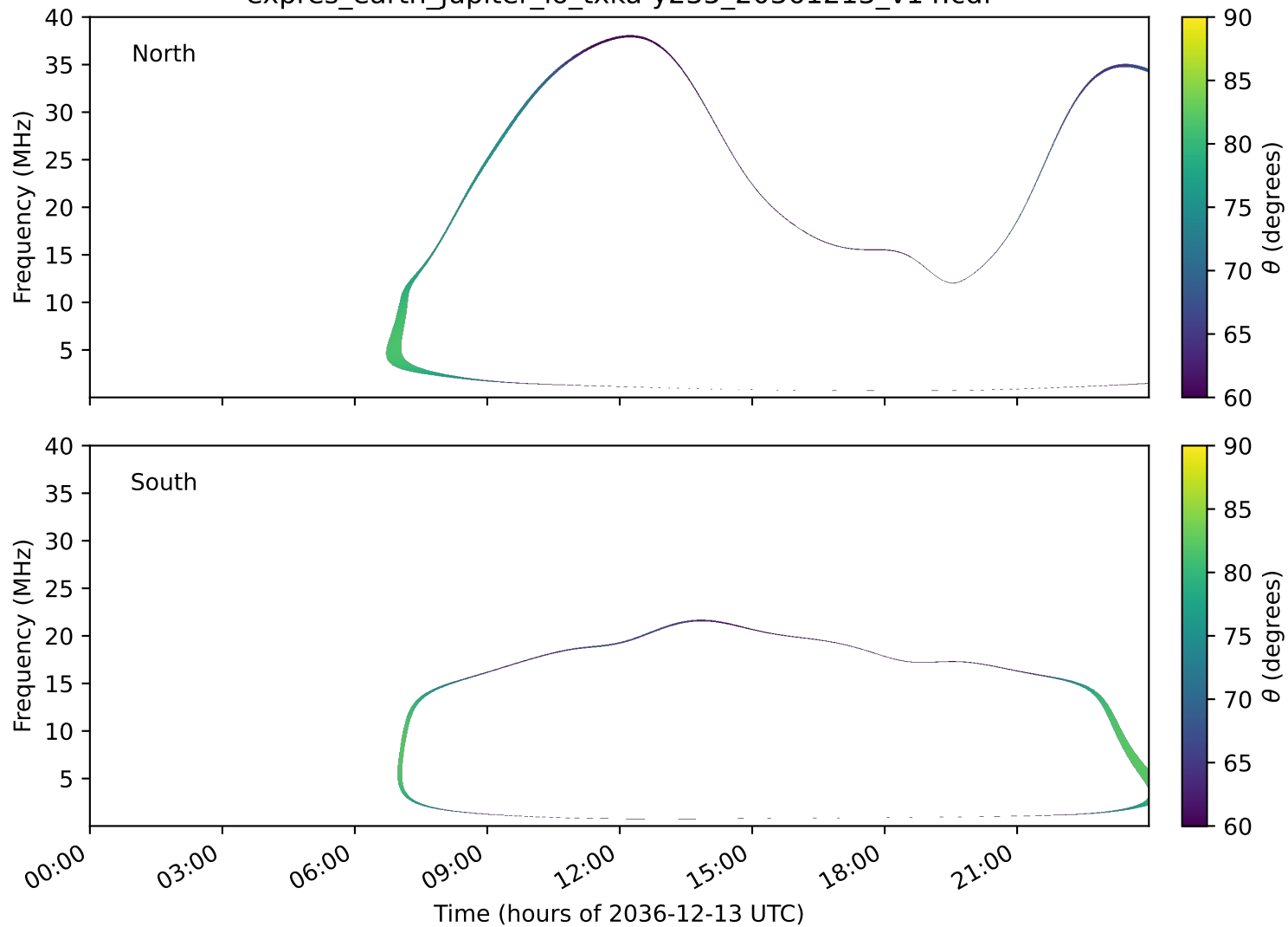
expres_earth_jupiter_io_txka-y235_20361213_v14.cdf
