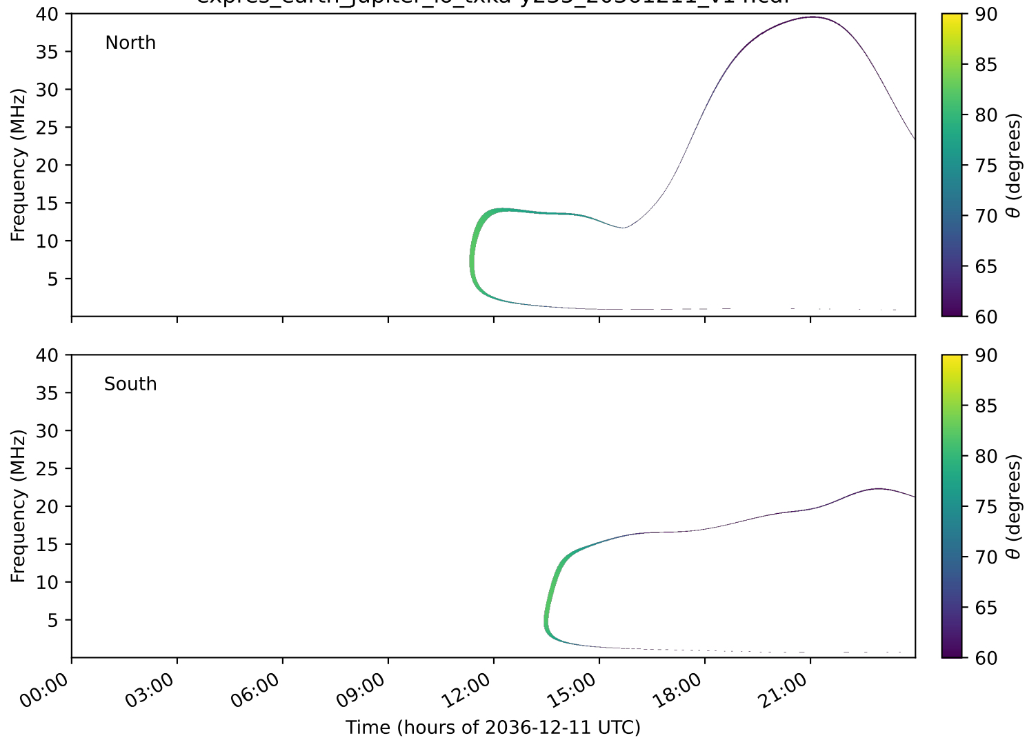
expres_earth_jupiter_io_txka-y235_20361211_v14.cdf
