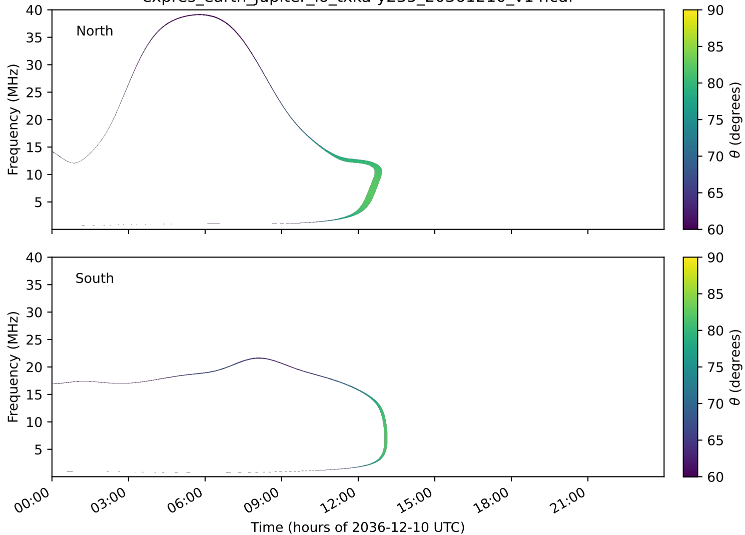
expres_earth_jupiter_io_txka-y235_20361210_v14.cdf
