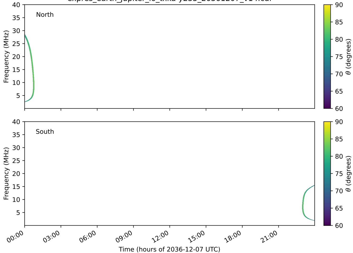
expres_earth_jupiter_io_txka-y235_20361207_v14.cdf
