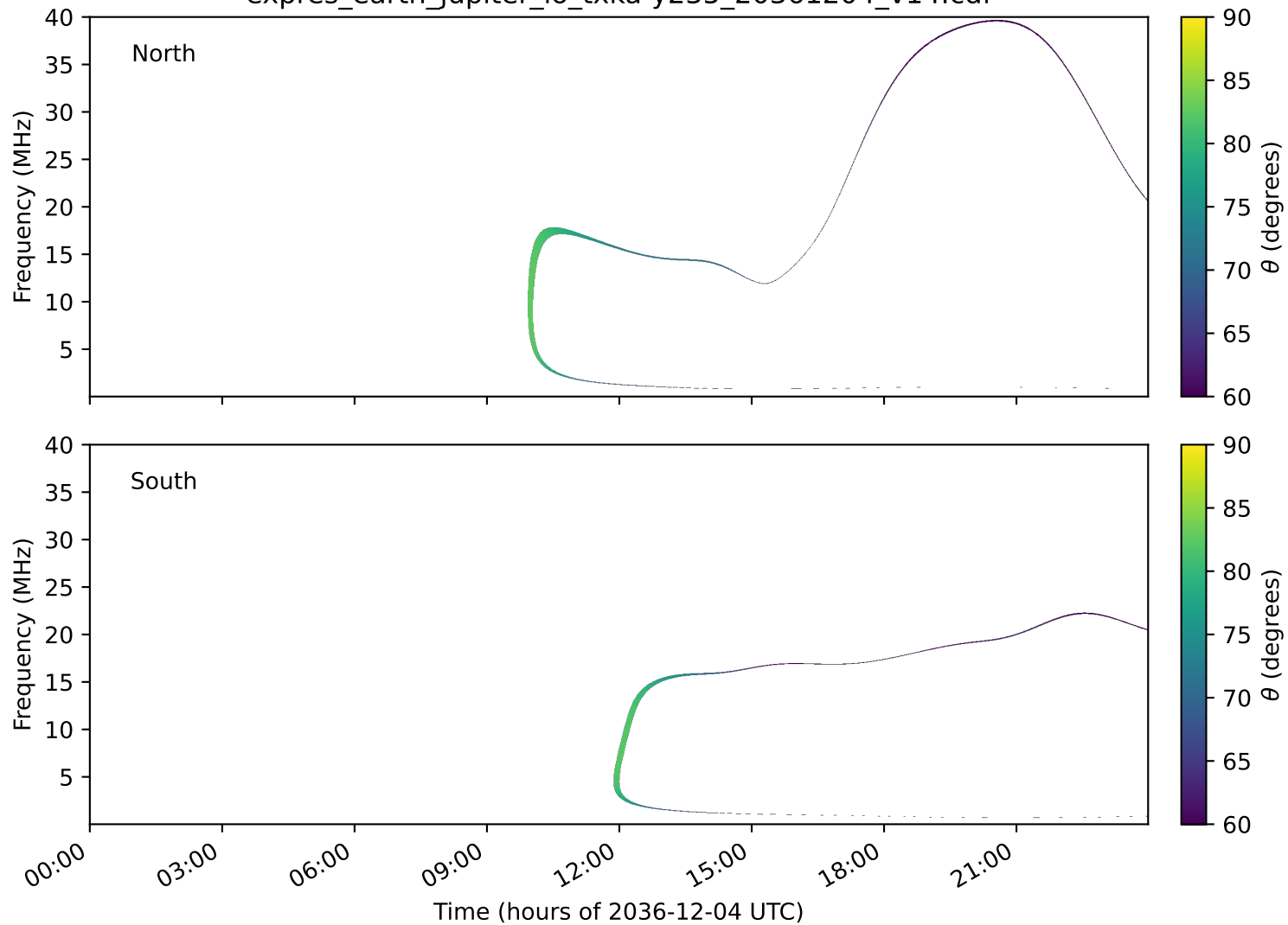
expres_earth_jupiter_io_txka-y235_20361204_v14.cdf
