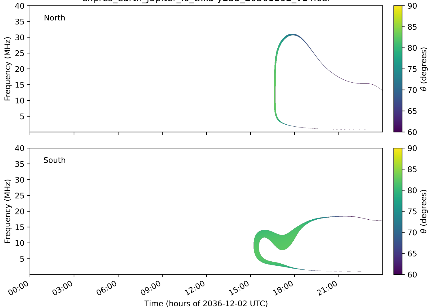
expres_earth_jupiter_io_txka-y235_20361202_v14.cdf
