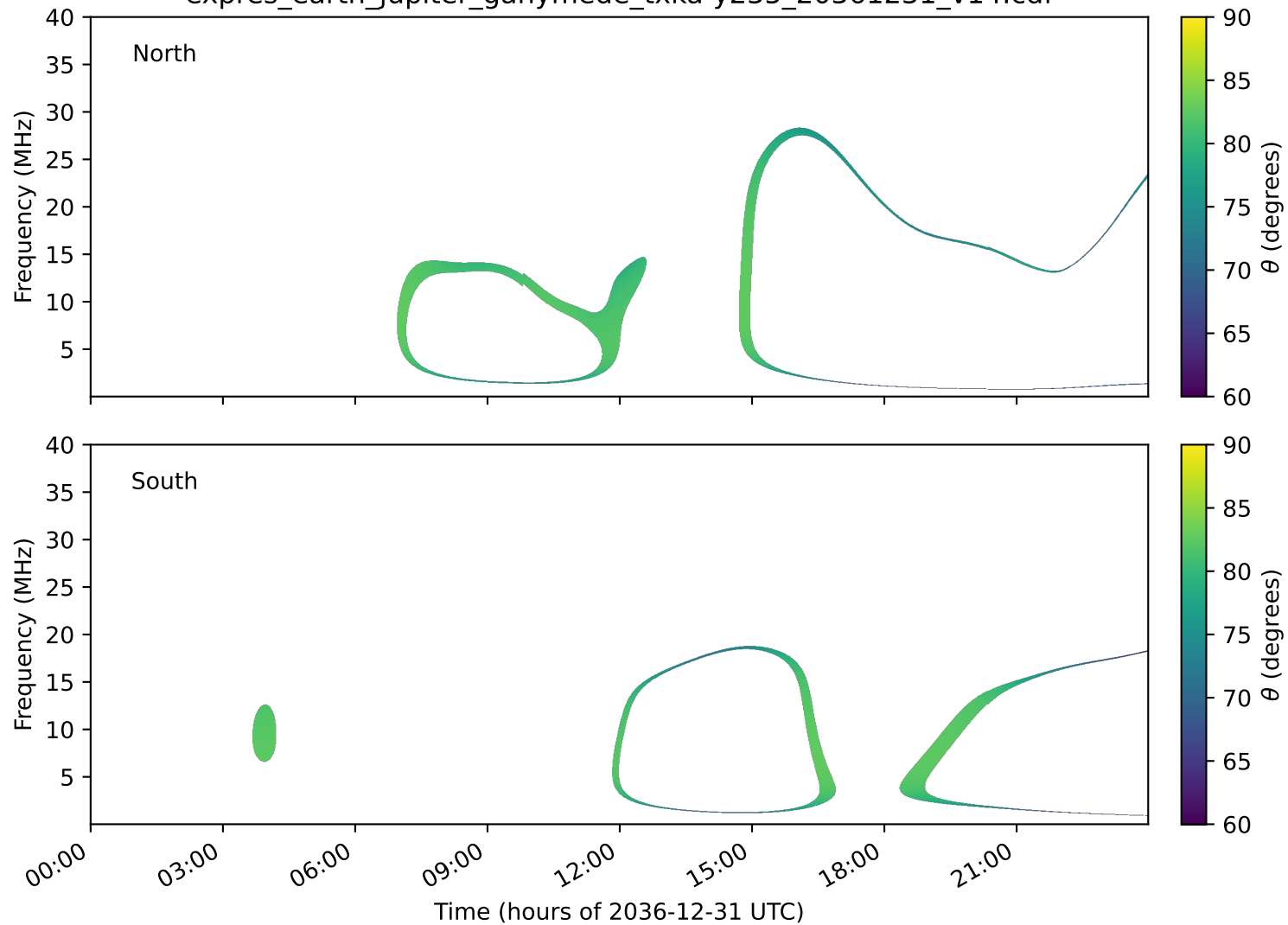
expres_earth_jupiter_ganymede_txka-y235_20361231_v14.cdf
