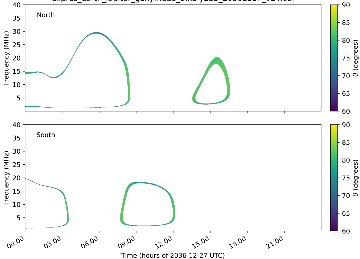
expres_earth_jupiter_ganymede_txka-y235_20361227_v14.cdf
