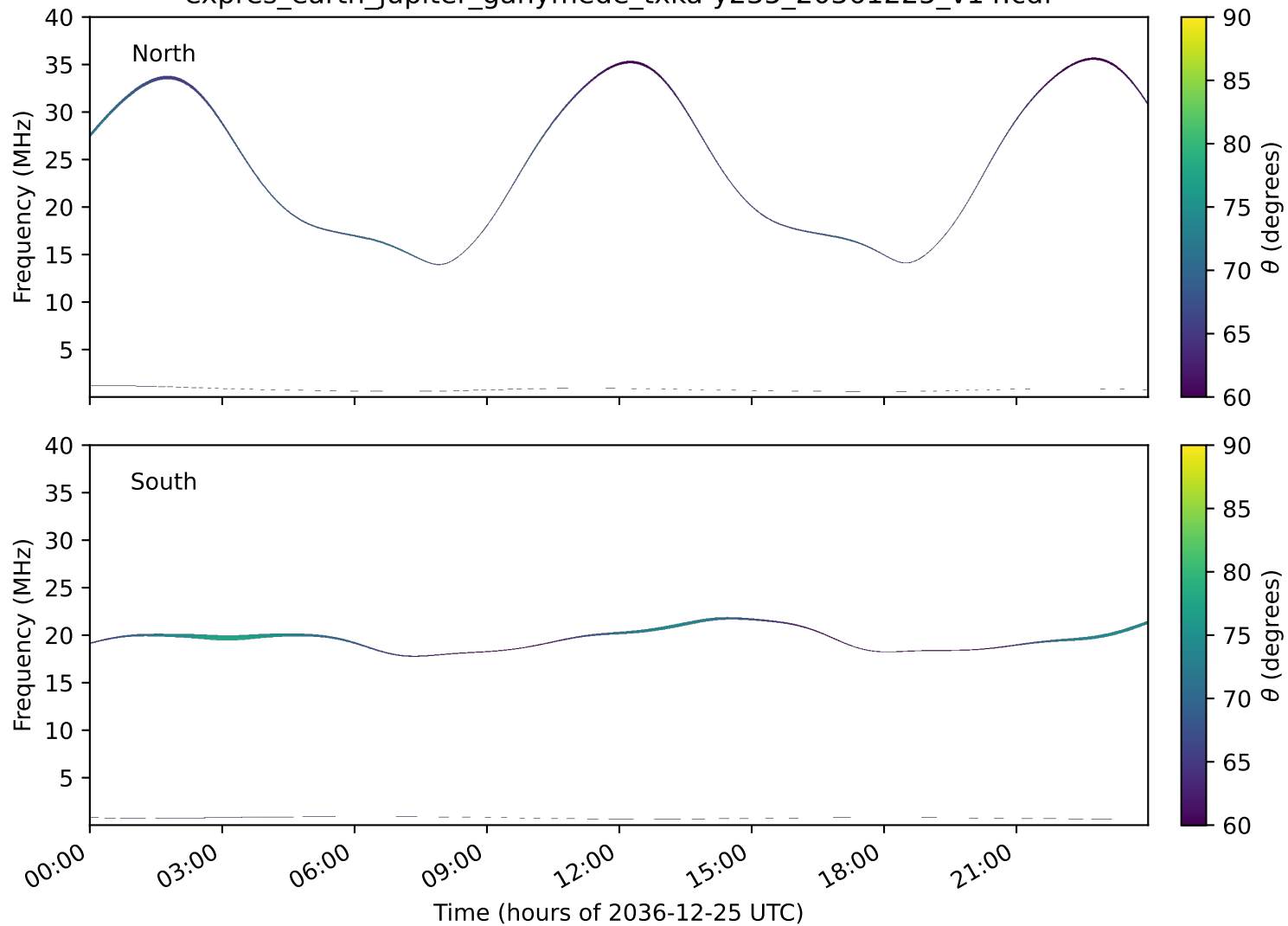
expres_earth_jupiter_ganymede_txka-y235_20361225_v14.cdf
