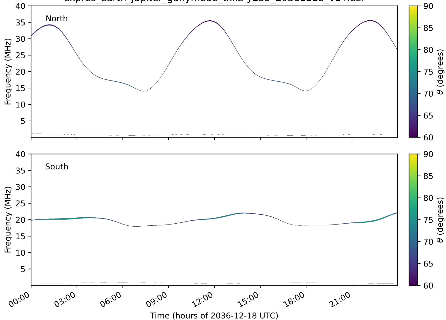
expres_earth_jupiter_ganymede_txka-y235_20361218_v14.cdf
