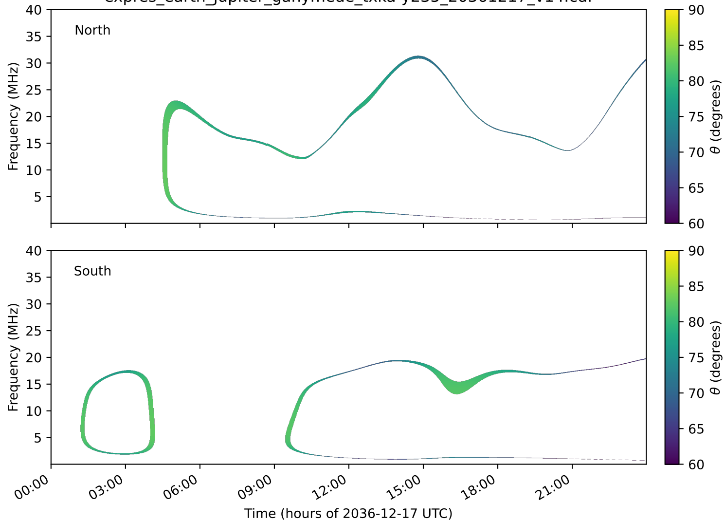
expres_earth_jupiter_ganymede_txka-y235_20361217_v14.cdf
