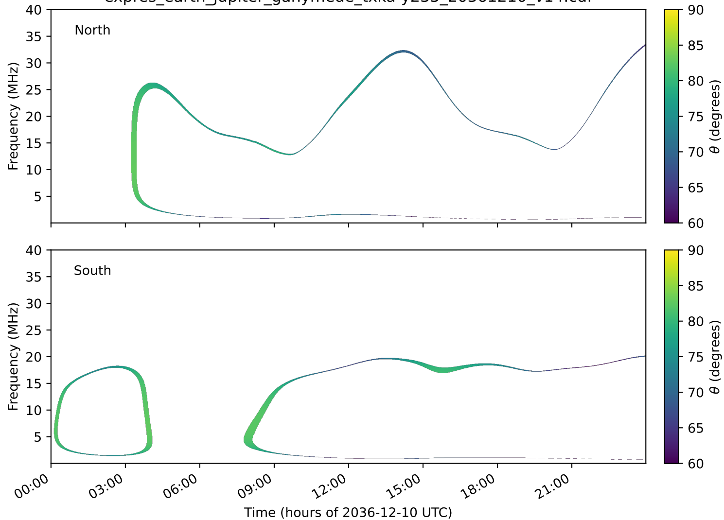
expres_earth_jupiter_ganymede_txka-y235_20361210_v14.cdf
