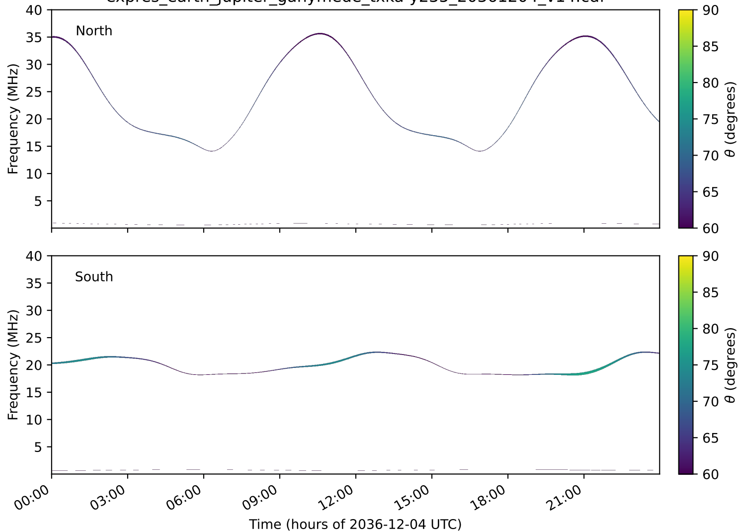
expres_earth_jupiter_ganymede_txka-y235_20361204_v14.cdf
