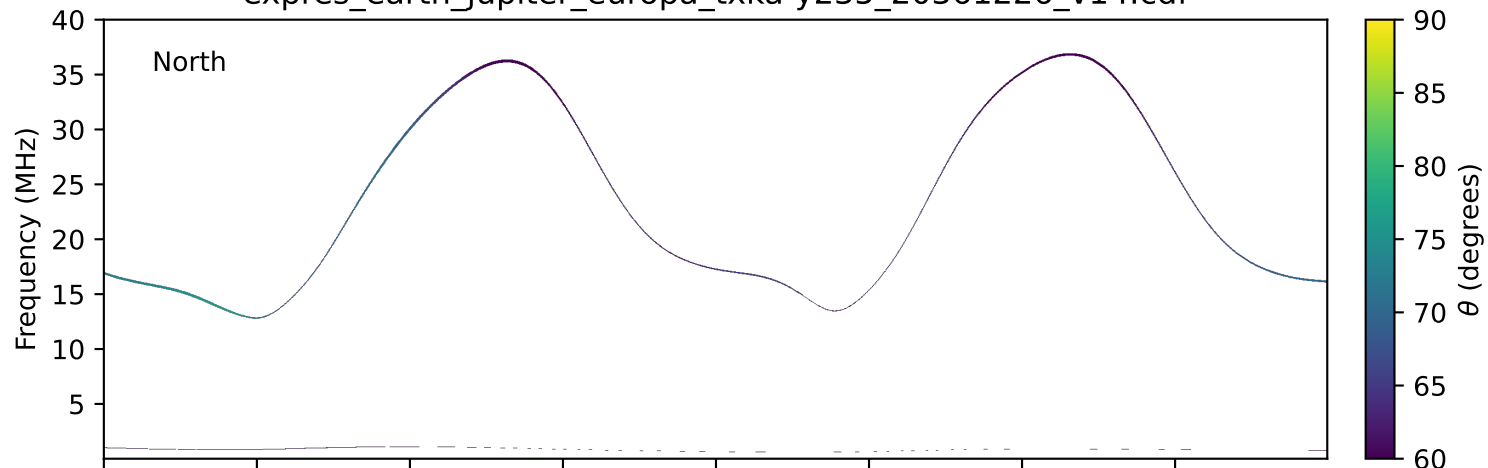
expres_earth_jupiter_europa_txka-y235_20361226_v14.cdf
