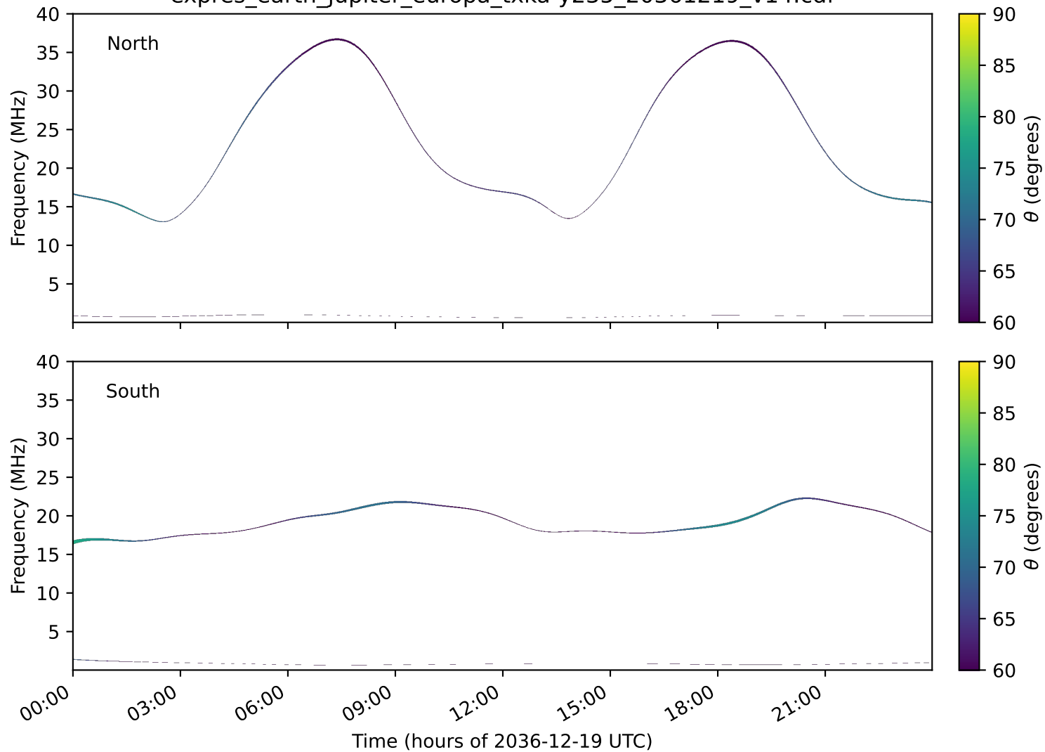
expres_earth_jupiter_europa_txka-y235_20361219_v14.cdf
