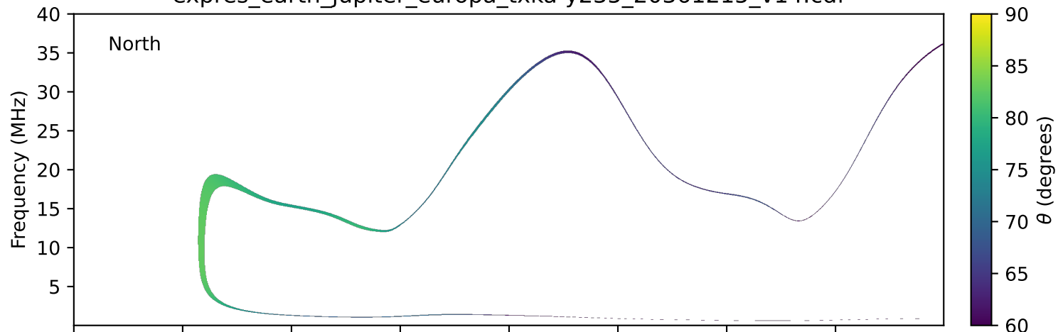
expres_earth_jupiter_europa_txka-y235_20361215_v14.cdf
