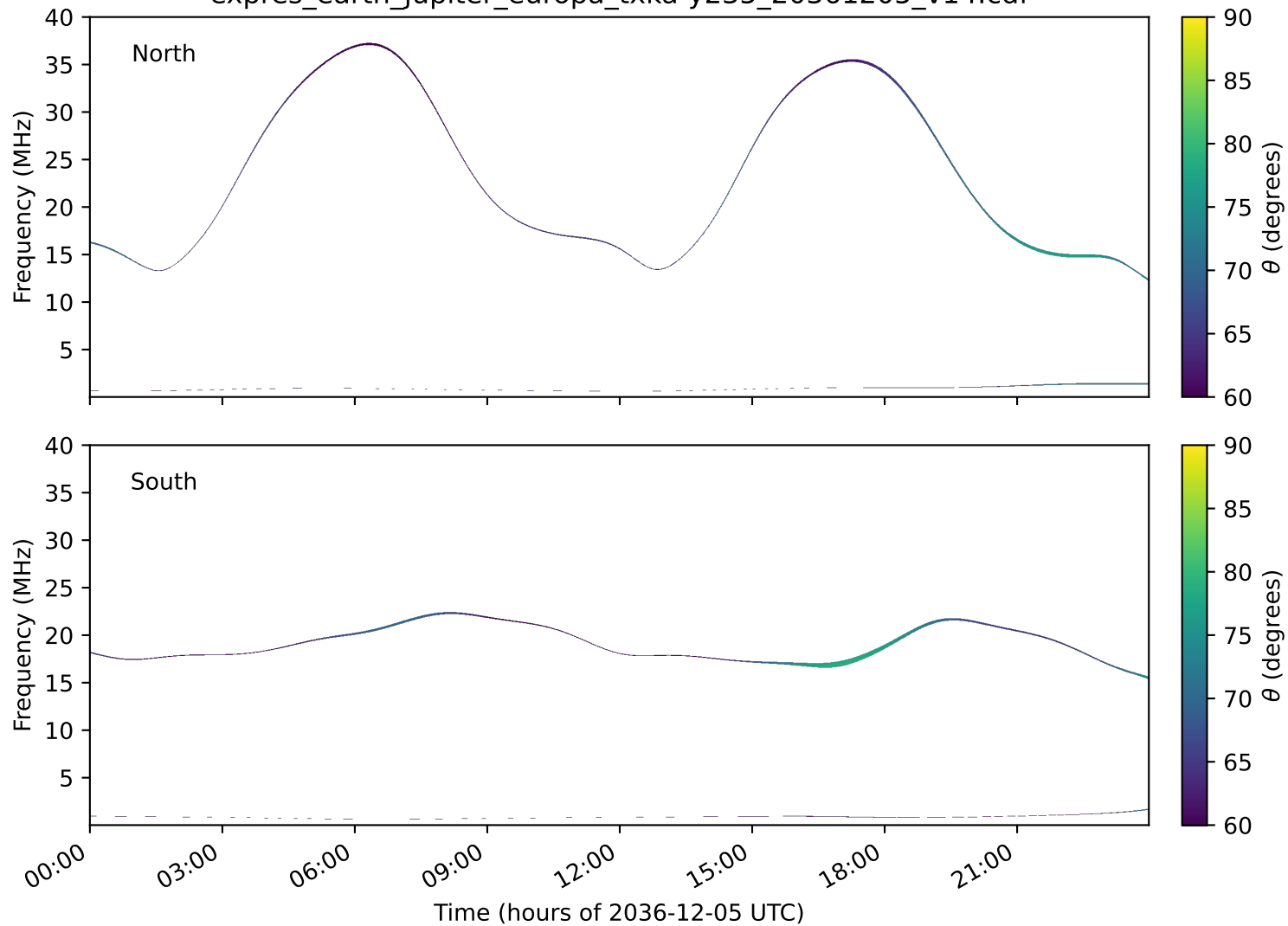
expres_earth_jupiter_europa_txka-y235_20361205_v14.cdf
