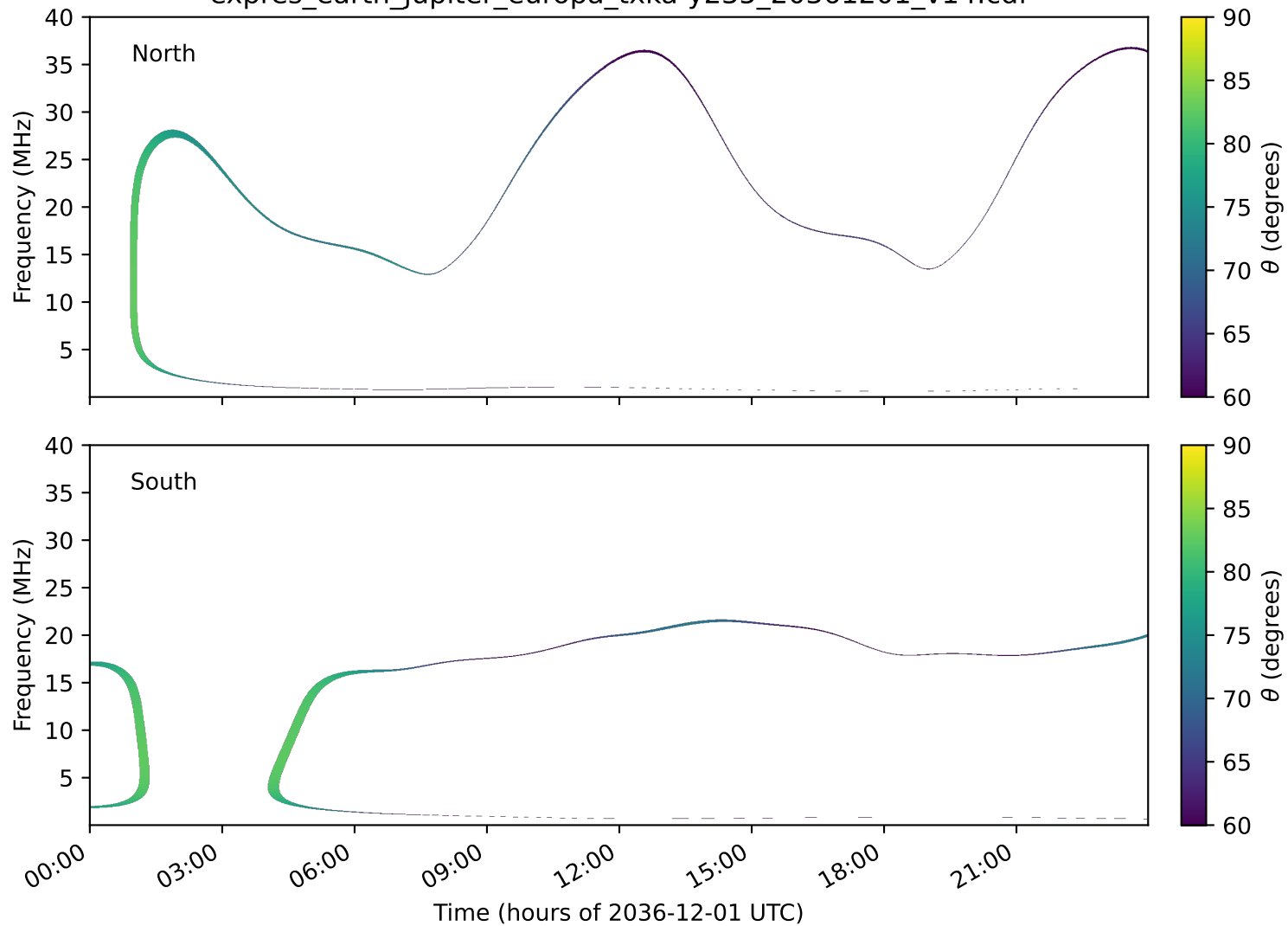
expres_earth_jupiter_europa_txka-y235_20361201_v14.cdf
