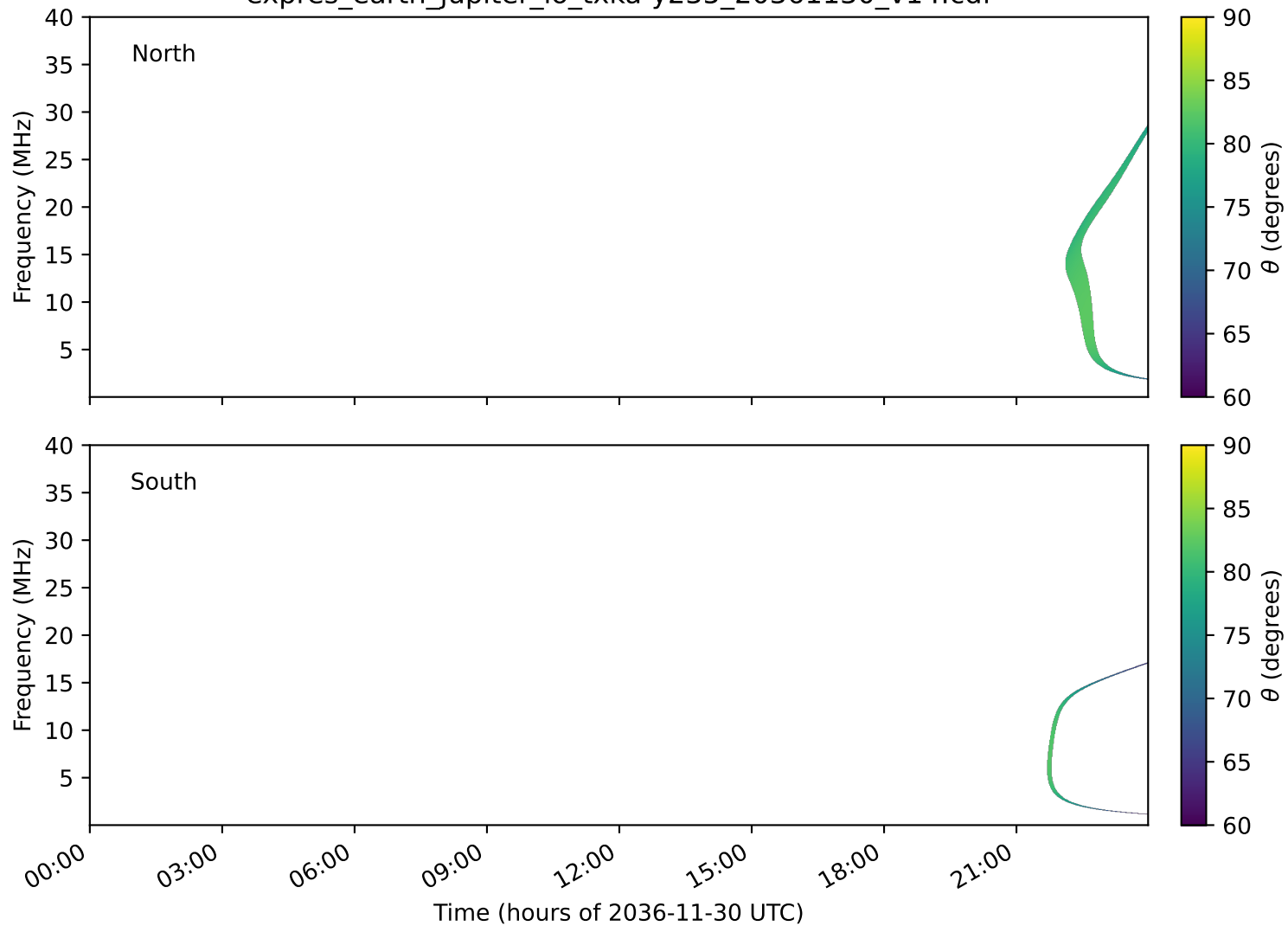
expres_earth_jupiter_io_txka-y235_20361130_v14.cdf
