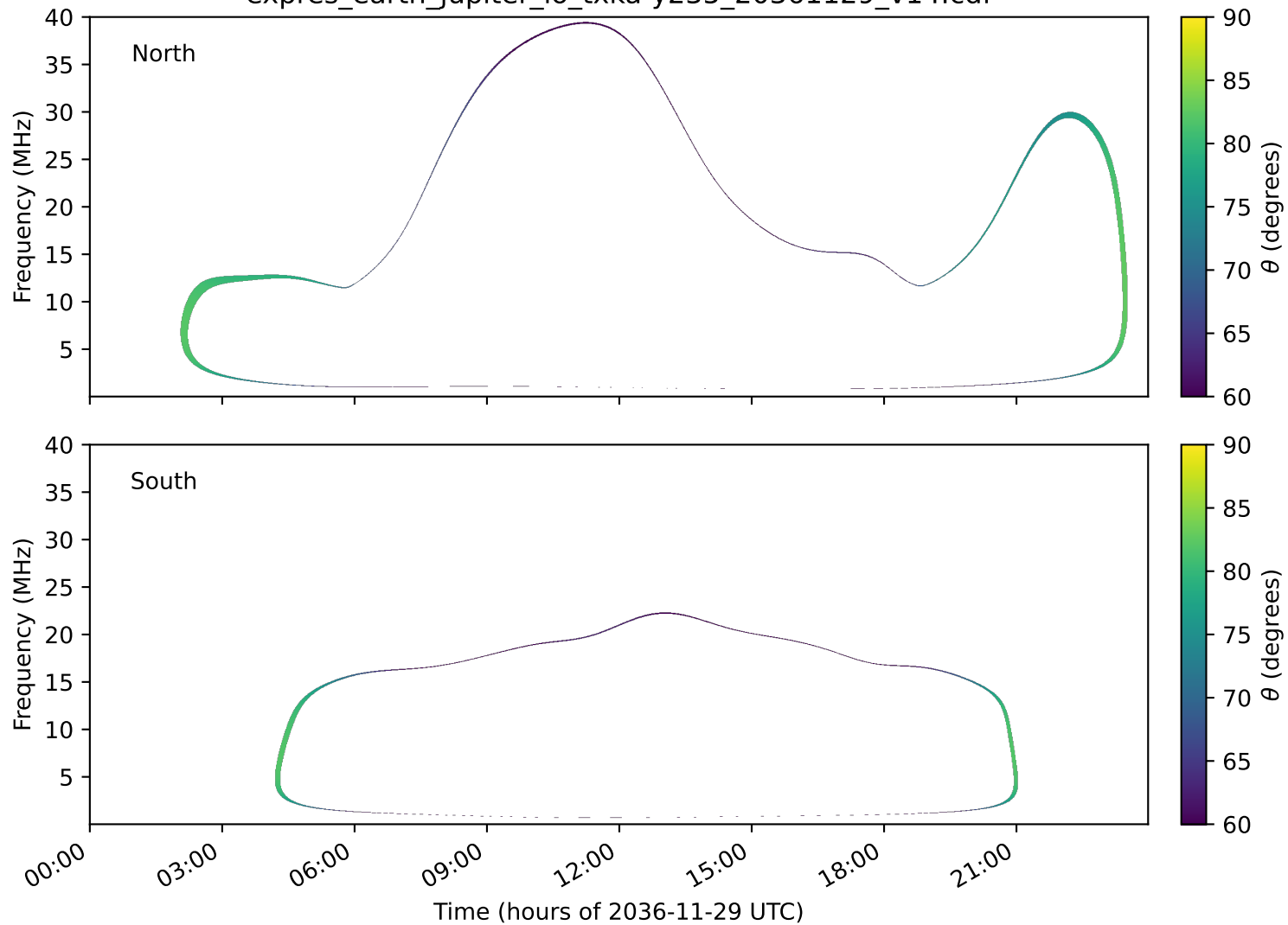
expres_earth_jupiter_io_txka-y235_20361129_v14.cdf
